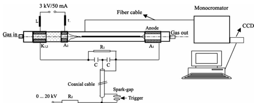
Figure 1. Experimental setup.
