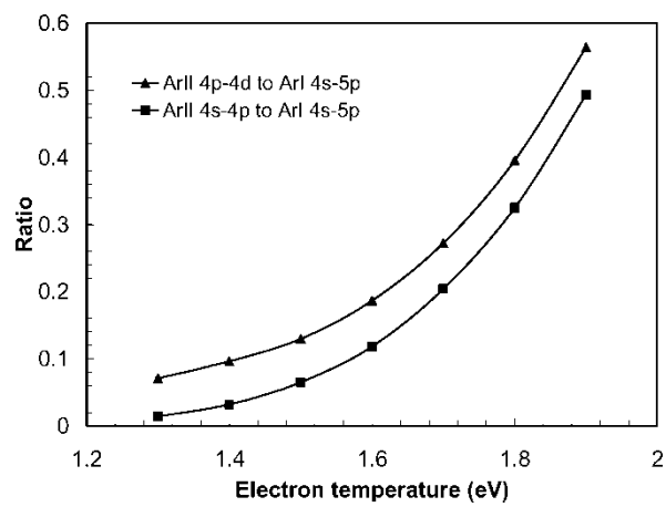
Figure 4. Line ratios of Ar(II) 4p-4d to Ar(I) 4s-5p line and Ar(II) 4s-4p to Ar(I) 4s-5p as function of electron temperature in eV.
