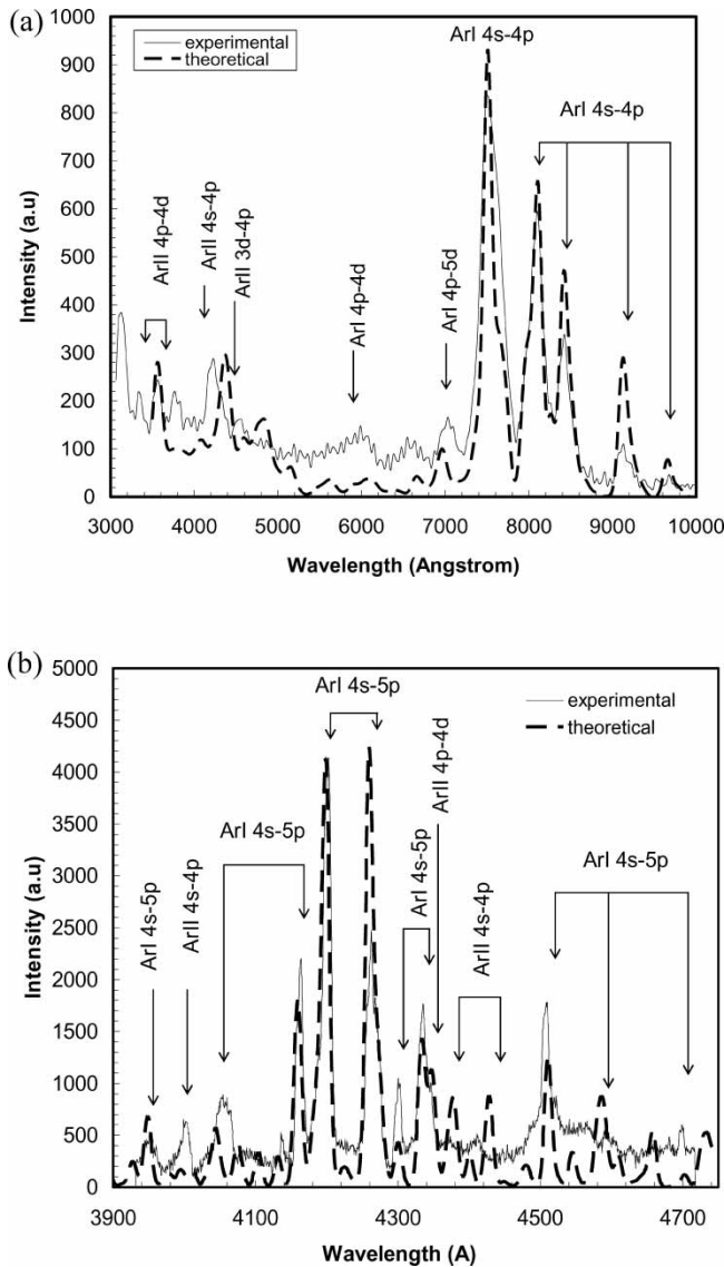
Figure 2. The experimental Ar(I) and Ar(II) spectrum from the glow discharge plasma superimposed on the theoretical spectrum: (a) spectrum between 300 nm and 1000 nm, (b) spectrum between 390 nm and 470 nm.
