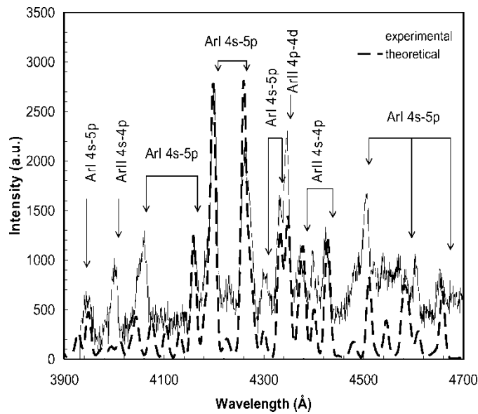
Figure 3. Experimental Ar(I) and Ar(II) spectra superimposed on theoretical spectra for the electron beam side at the generator; region between A_1 and A_2 .
